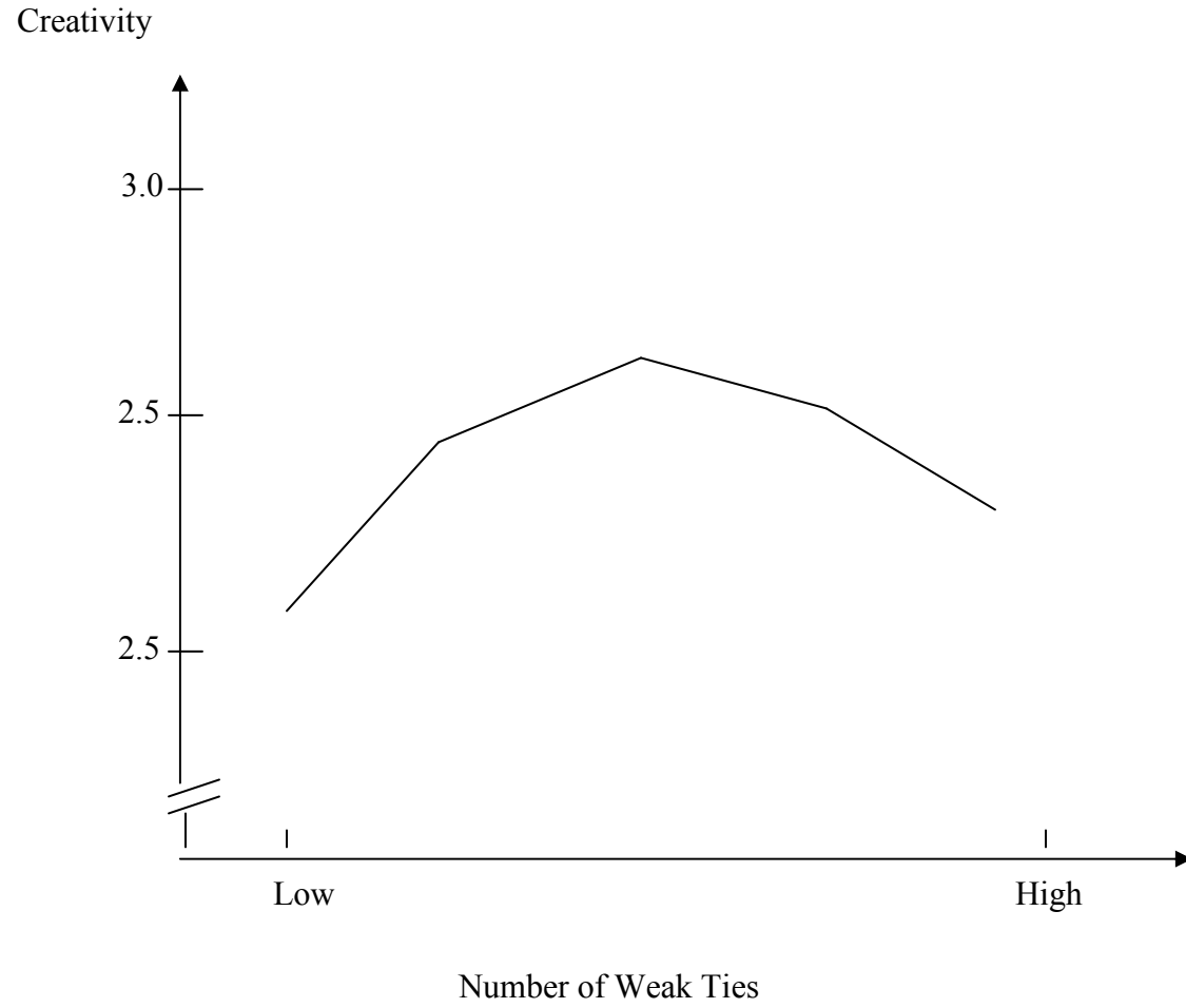
Curvilinear Relationship between Number of Weak Ties and Creativity
