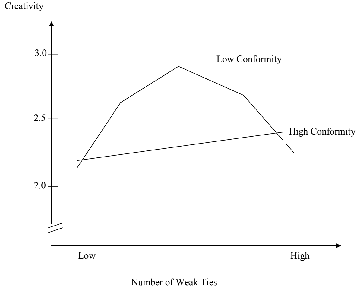
Curvilinear by Linear Relationship between Number of Weak Ties, Conformity and Creativity
